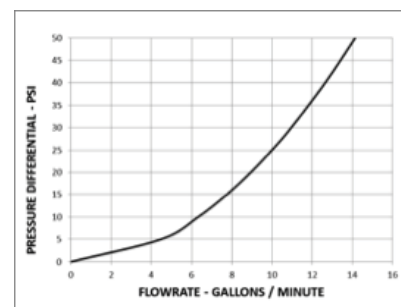
Note: Flow rate determined on a Heatguard® 110-D LF with 1/2" sweat fittings
